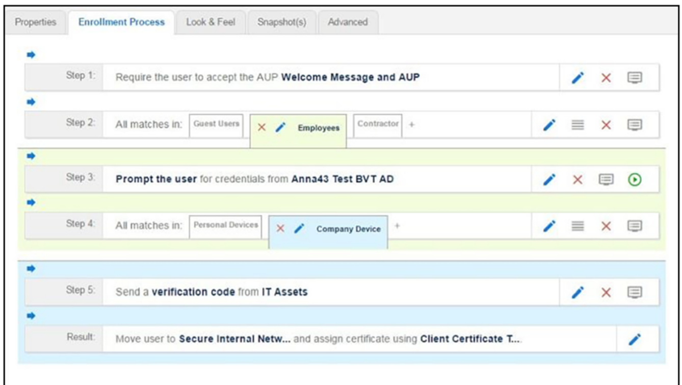
FIGURE 41 Workflow with Device Ownership Split
