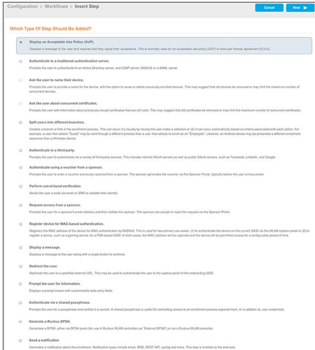
FIGURE 37 Enrollment Step Selection
